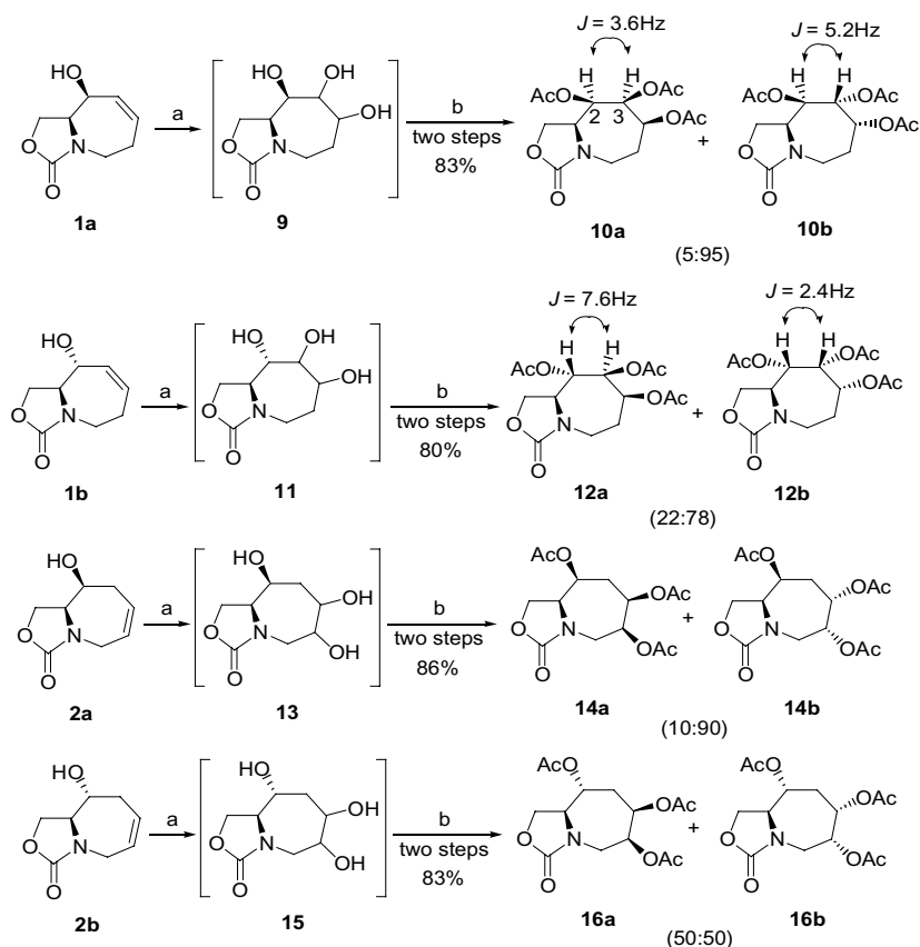
Scheme 2. Dihydroxylation of oxazolidinyl azacycles. Reagents and conditions: (a) \text{OsO}_4 , NMO, acetone/ \text{H}_2\text{O} = 8:1; (b) \text{Ac}_2\text{O} , py, DMAP, \text{CH}_2\text{Cl}_2 , rt, two steps 80%.
