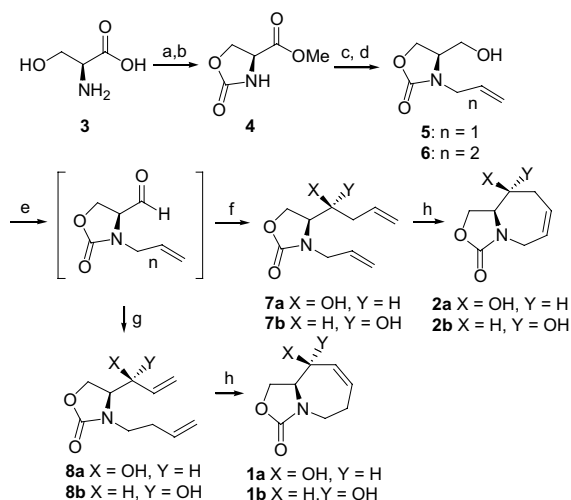
Scheme 1. Synthesis of oxazolidinyl azacycles. Reagents and conditions: (a) \text{SOCl}_2 , MeOH reflux, overnight; (b) \text{K}_2\text{CO}_3 , triphosgene, \text{H}_2\text{O} /toluene, 87%; (c) 60% NaH, allyl bromide or homoallyl bromide, DMF; (d) \text{NaBH}_4 , MeOH; (e) DMSO, (\text{COCl})_2 , \text{CH}_2\text{Cl}_2 , \text{Et}_3\text{N} ; (f) allylmagnesium bromide; (g) vinylmagnesium bromide; (h) Grubb's catalyst (10 mol%), \text{CH}_2\text{Cl}_2 , reflux, 12 h.
